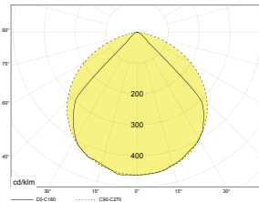
LOR 100% Total flux 15945lm SHRnom 1.25 SHRmax 1.379
