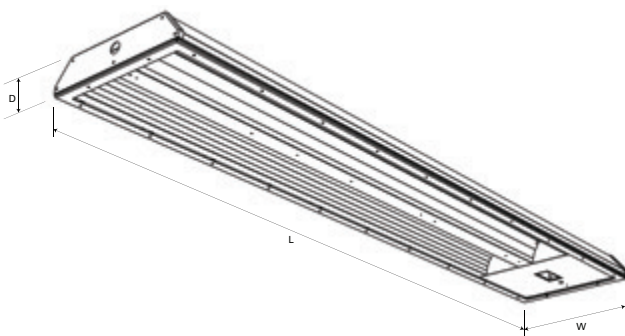
LOR 100% Total flux 15684lm SHRnom 1.00 SHRmax 1.141
