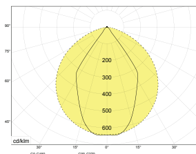
LOR 100% Total flux 15684lm SHRnom 1.00 SHRmax 1.141
