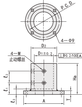
●圆法兰支架
